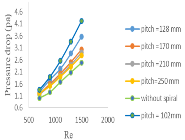
Fig 7 Pressure drop variation for different Re for height 5 mm & different pitches.
