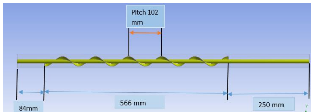
Fig 1 Computational domain and Boundaries
