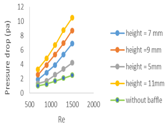
Fig 9 Pressure drop variation for different Re for height 5 mm & different pitches.
