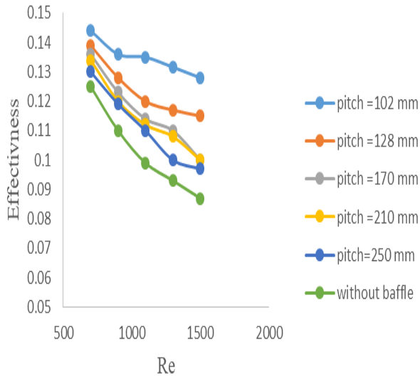
Fig 10 Effectiveness variation for different Re for pitch 102 mm & different height.
