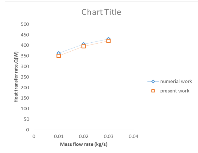
Fig 2 Heat transfer rate variation for different mass flow rate.
