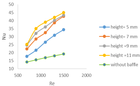
Fig 6 Nusselt number variation for different Re for pitch 102 mm & different height.
