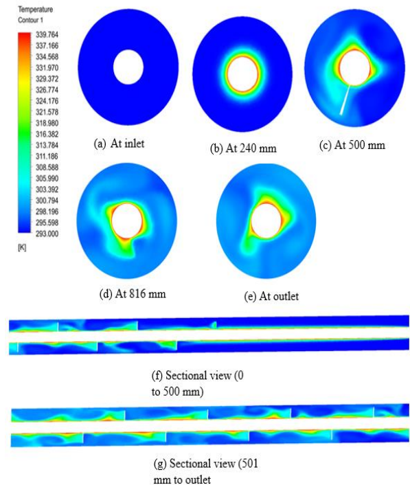
Fig 4 Temperature contours for different positions in annulus side for pitch 102 mm with height 11 mm
