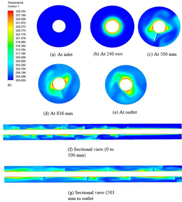
Fig 3 Temperature contours for different positions in annulus side for pitch 102 mm with height 9 mm.
