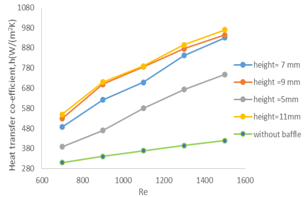
Fig 8 Heat transfer co-efficient variation for different Re for pitch 102 mm & different height.
