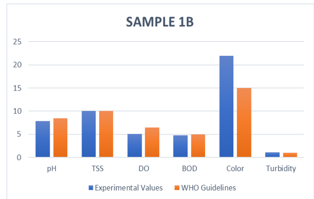
Figure 03: Comparison of pH, TSS, DO, BOD, Color, and Turbidity of sample 01 between Experimental Values and WHO Guidelines
