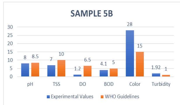
Figure 11: Comparison of pH, TSS, DO, BOD, Color, and Turbidity of sample 05 between Experimental Values and WHO Guidelines
