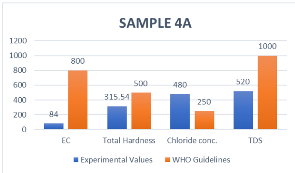
Figure 08: Comparison of EC, TH, Cl - and TDS of sample 04 between Experimental Values and WHO Guidelines
