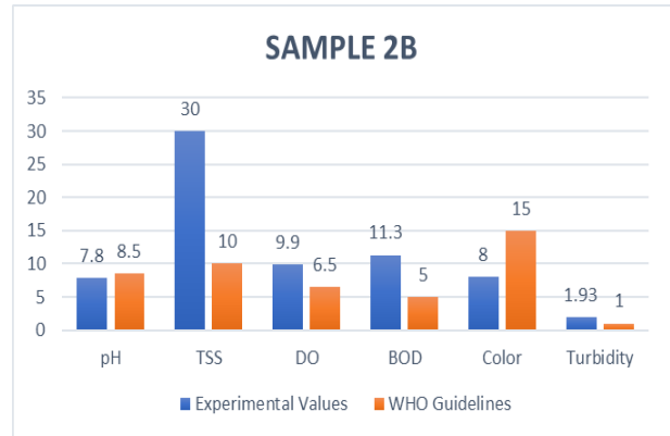
Figure 05: Comparison of pH, TSS, DO, BOD, Color, and Turbidity of sample 02 between Experimental Values and WHO Guidelines
