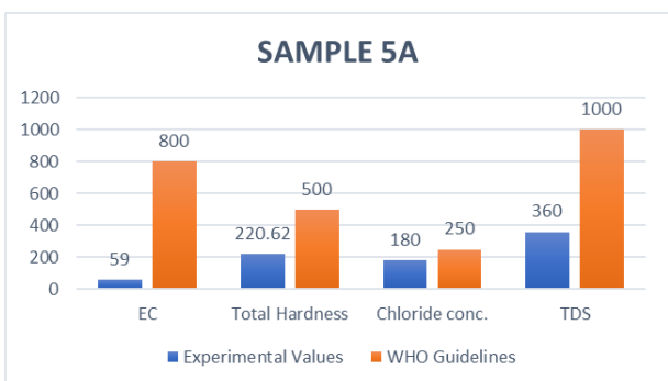
Figure 10: Comparison of EC, TH, Cl - and TDS of sample 05 between Experimental Values and WHO Guidelines
