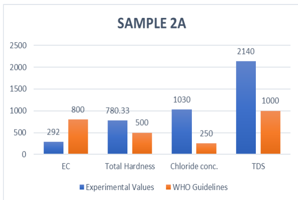
Figure 04: Comparison of EC, TH, Cl - and TDS of sample 02 between Experimental Values and WHO Guidelines
