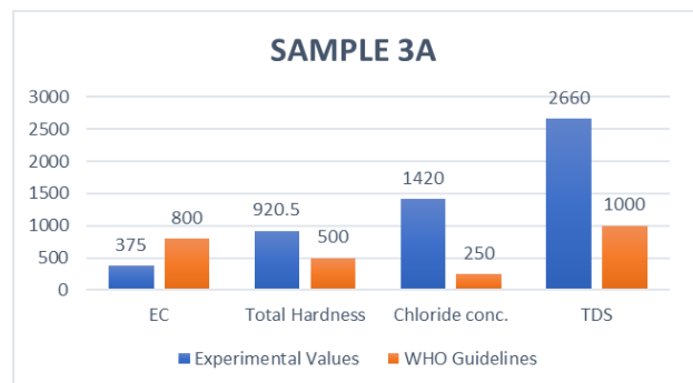
Figure 06: Comparison of EC, TH, Cl - and TDS of sample 03 between Experimental Values and WHO Guidelines.
