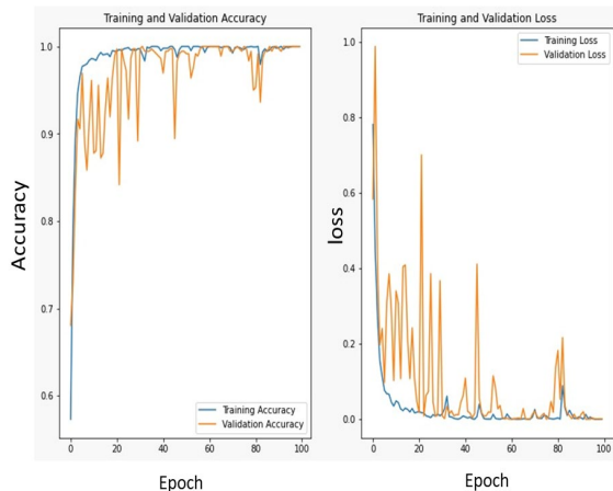
Fig. 7 Accuracy and loss curve of CNN
