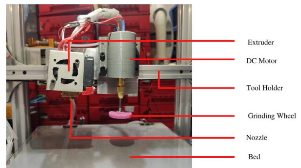
Fig.6 Hybrid machining setup
