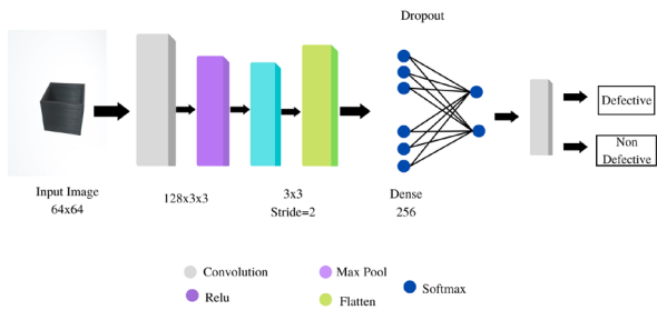
Fig. 4: Architecture of convolutional neural network
