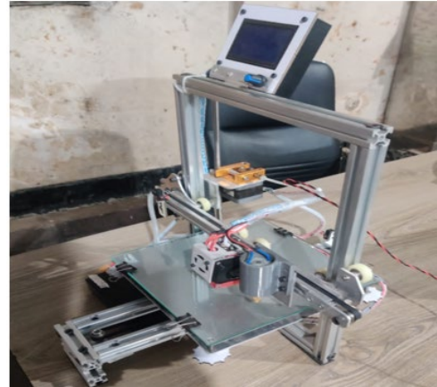
Fig. 5 Hybrid Manufacturing Machine
