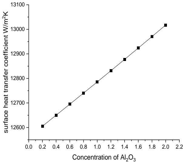
Fig.13: Change of heat transfer coefficient, h for different volume fraction in hot and cold
