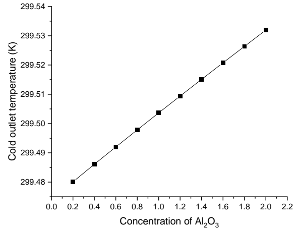
Fig.11. Cold outlet temperature vs Volume fraction
