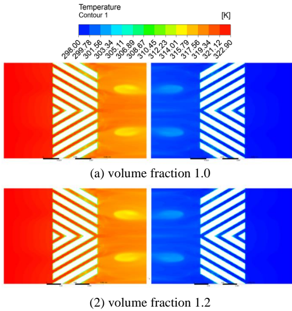
Fig.9: Temperature contour for Reynolds number 10000 for volume fraction (1)1.0 and (2) 1.2 in Hot Outlet and Cold Outlet
