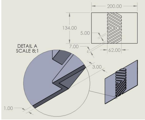
Fig.2 Dimensions of the geometry
