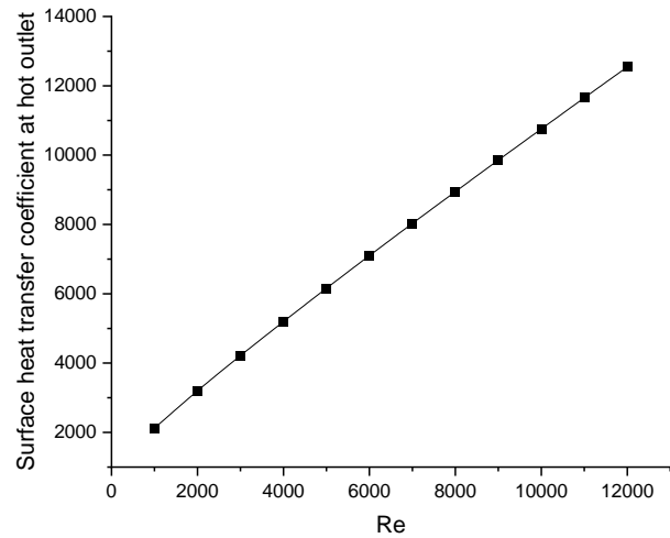
Fig.7: Change of heat transfer coefficient (h) of hot outlet along with Reynolds number
