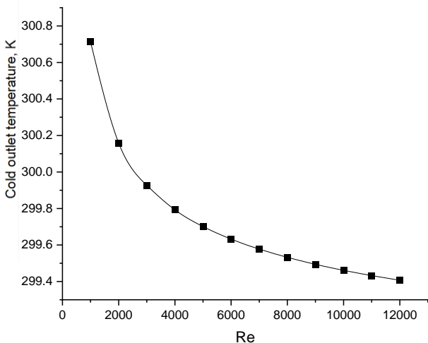
Fig.6: Cold outlet temperature vs Reynolds number
