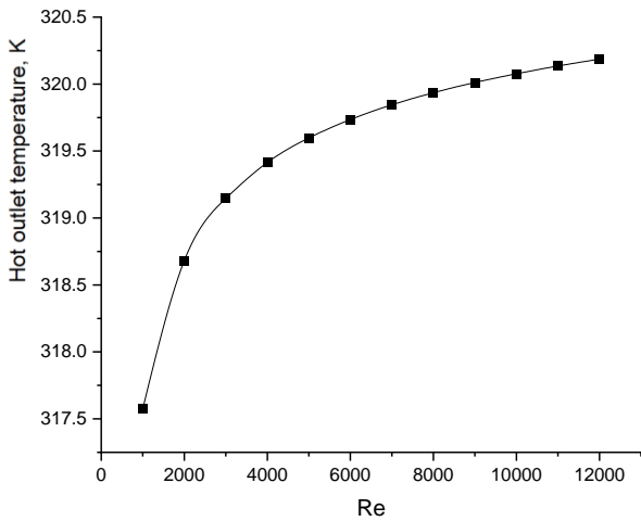
Fig.5: Hot outlet temperature vs Reynolds number
