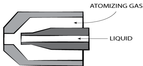
Fig.1 Air blast type twin fluid atomizer [3].
