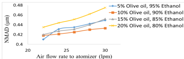
Fig.11 Effect of air flow rate to atomizer on NMAD for different composition for 56.6 lpm air flow rate to virtual impactor.
