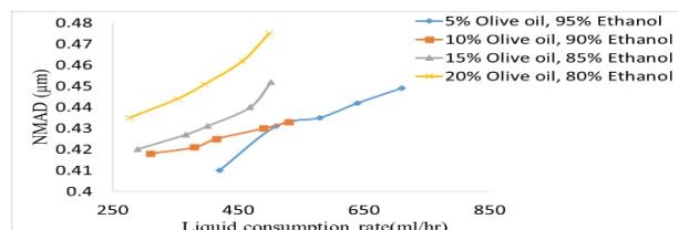
Fig.9 Effect of liquid consumption rate on NMAD for different composition for 56.6 lpm air flow rate to virtual impactor.
