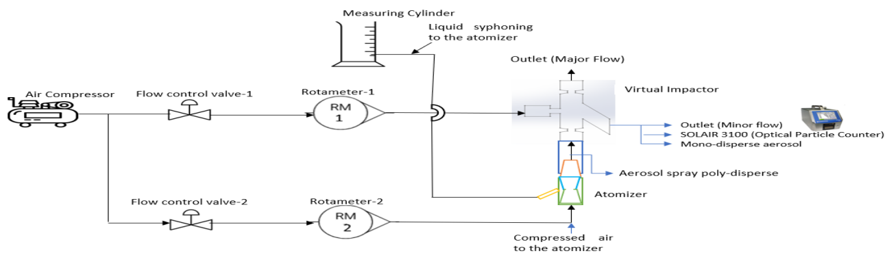
Fig.7 Schematic diagram of Experimental Setup for producing mono-disperse aerosol using the designed virtual impactor.
