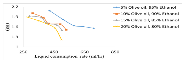
Fig.8 Effect of liquid consumption rate on GSD for different composition for 56.6 lpm air flow rate to virtual impactor.
