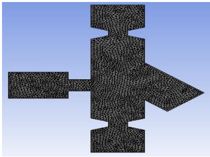
Fig.4 Mesh of the virtual impactor.
