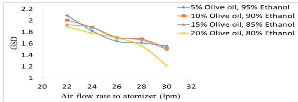
Fig.10 Effect of air flow rate to atomizer on GSD for different composition for 56.6 lpm air flow rate to virtual impactor.
