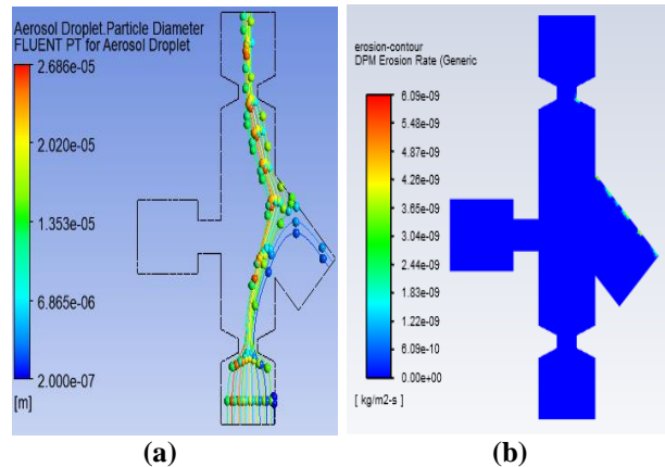
Fig.6 (a) Aerosol particle tracking and (b) erosion contours of the virtual impactor.
