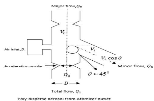
Fig.3 Simplified Impactor Model with circular area of major flow and minor flow.
