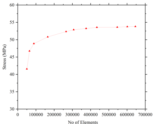
Fig.4 Mesh sensitivity analysis
