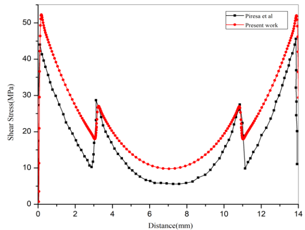
Fig.5 Comparison of shear stress with pires et al.
