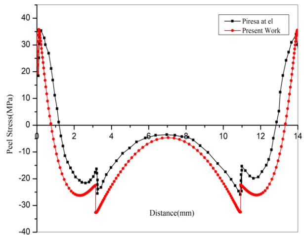
Fig.6 Comparison of peel stress with pires et al.
